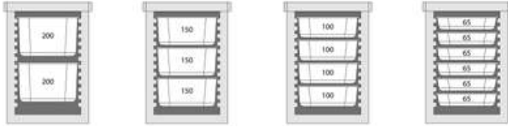
2x GN1/1 200 mm 3x GN1/1 150 mm 4x GN1/1 100 mm 6x GN1/1 65 mm
